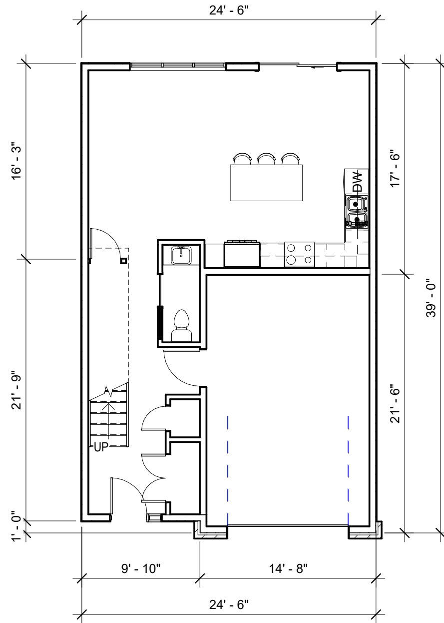
① TOWNHOME 1 LEVEL 1 1/8" = 1'-0"
