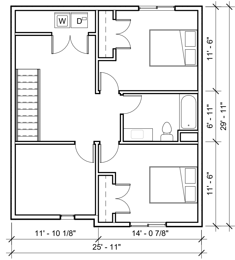
① 2 Car Townhome 3 level 3 Schematic 1/8" = 1'-0"
