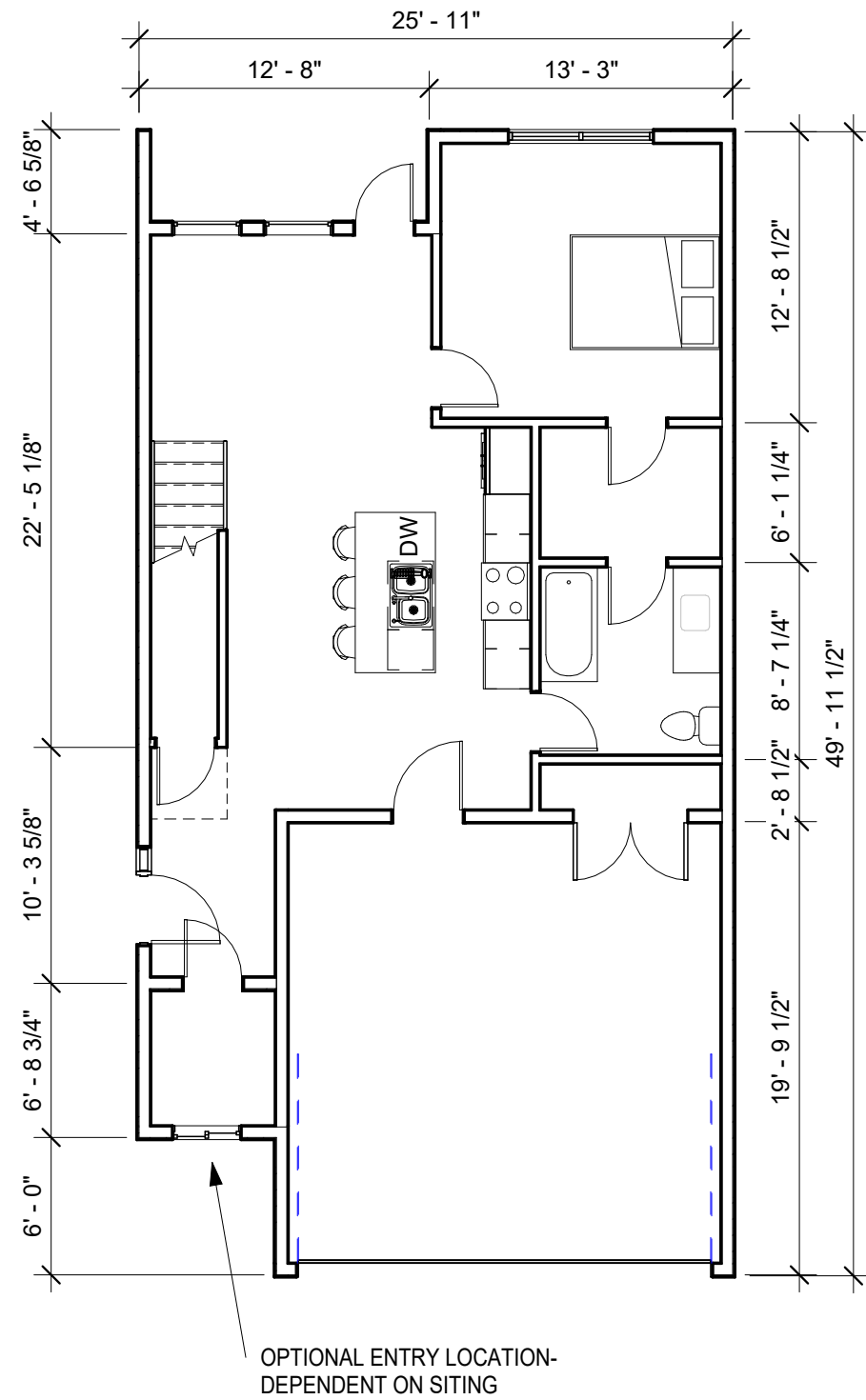
① TOWNHOME 6 LEVEL 1 1/8" = 1'-0"
