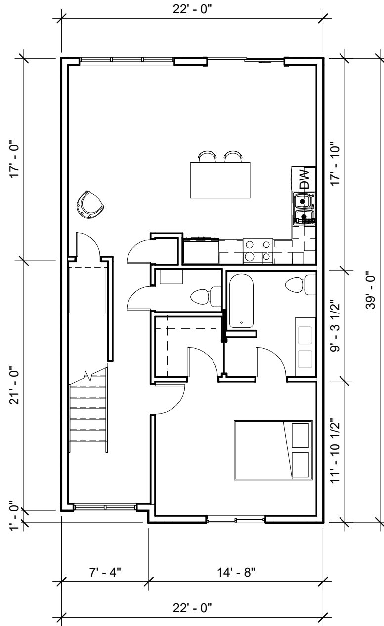
② TOWNHOME 3 LEVEL 2 1/8" = 1'-0"
