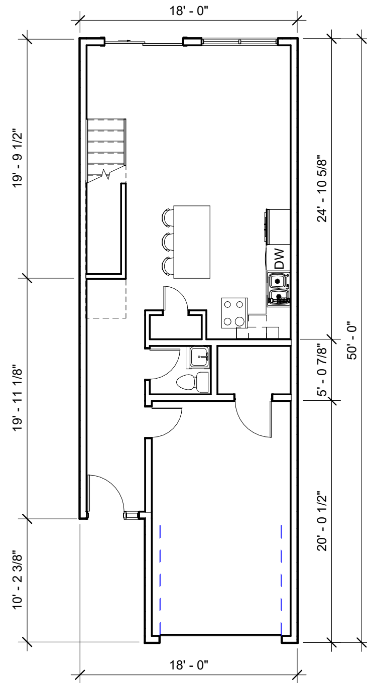
① TOWNHOME 2B LEVEL 1 1/8" = 1'-0"
