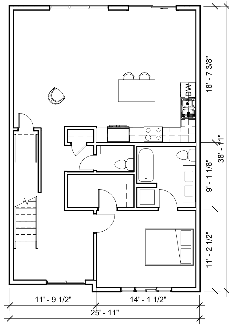
② 2 Car Townhome 3 Level 2 Schematic 1/8" = 1'-0"
