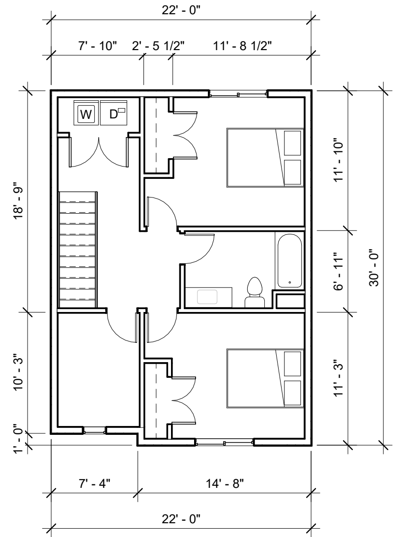
③ TOWNHOME 3 LEVEL 3 1/8" = 1'-0"
