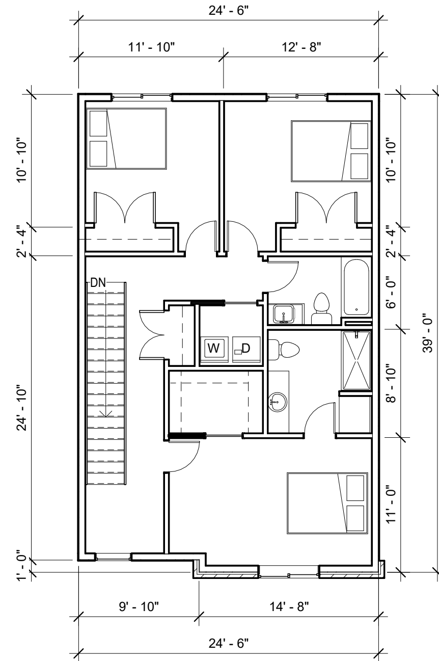
② TOWNHOME 1 LEVEL 2 1/8" = 1'-0"
