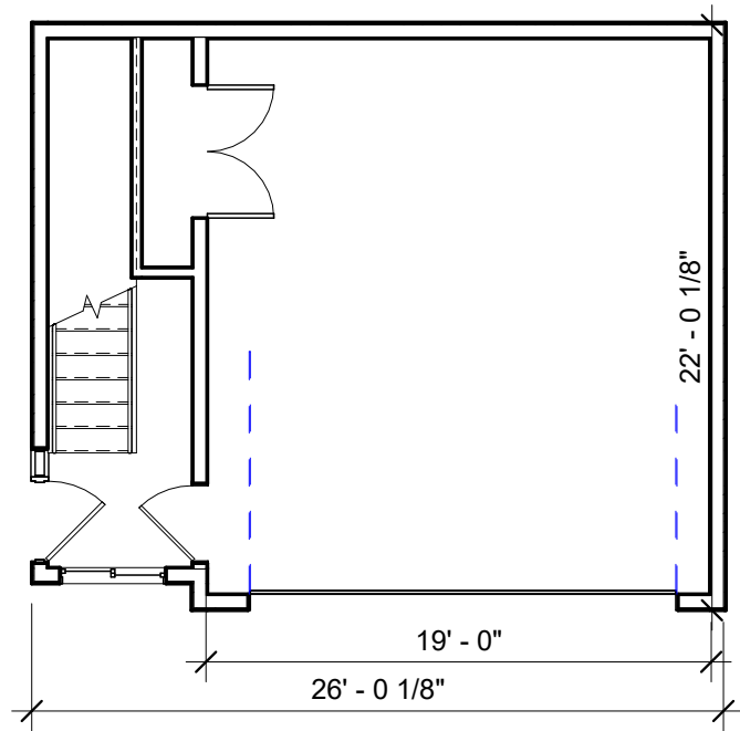
③ 2 Car Townhome 3 Level Schematic 1/8" = 1'-0"
